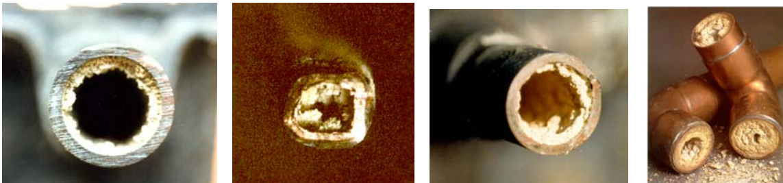
Oahu Solar Collector Panel Tubing 4 to 8 years old WITHOUT Water Softening
