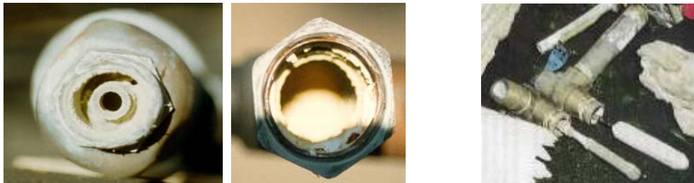
Oahu Solar Pressure Relief Valves 4 to 8 years old WITHOUT Water Softening
